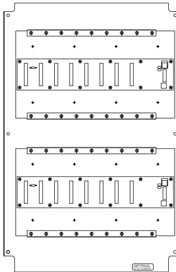
Figure 3. Two I/O Module Card Cages with Provision for Two I/O Motherboards (P/N 74-200000-008)
