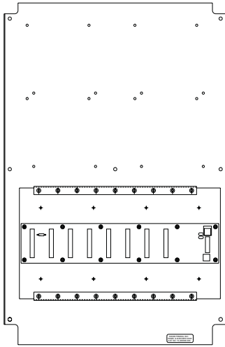
Figure 1. I/O Module Card Cage with Provisions for One I/O Motherboard and Four Power Supply Modules (P/N 74-200000-006)
