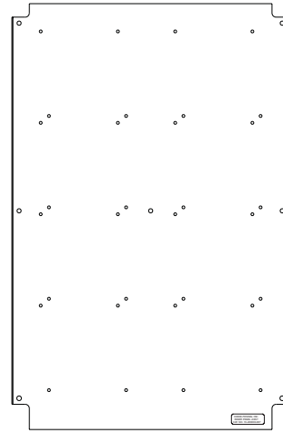
Figure 2. Up to Eight Power Supply Modules (P/N 74-200000-007)
