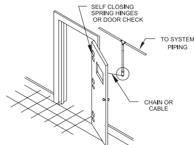
SWINGING DOOR-SELF CLOSING
